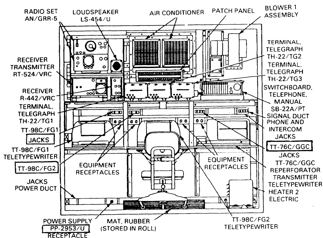
FRONT WALL
